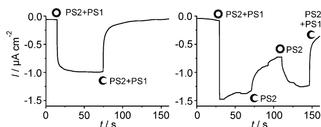
Figure 3. Photocurrent density of the proposed biophotovoltaic cell combining the PS2/Os1-based photoanode and the PS1/Os2-based photocathode as shown in Figure 2. The light status of the respective photoelectrode is indicated by O = light on and C = light off. Left: Simultaneous illumination of both half-cells with the same light intensity. Right: Starting with the same light intensity on both sides, light at the PS2 half-cell is switched off after 75 s and on again 30 s later. Finally, light was switched off at both half-cells. (Photoanode compartment: buffered electrolyte pH 6.5 ; photocathode compartment: buffered electrolyte pH 5.5 containing 2 mM methyl viologen.)
